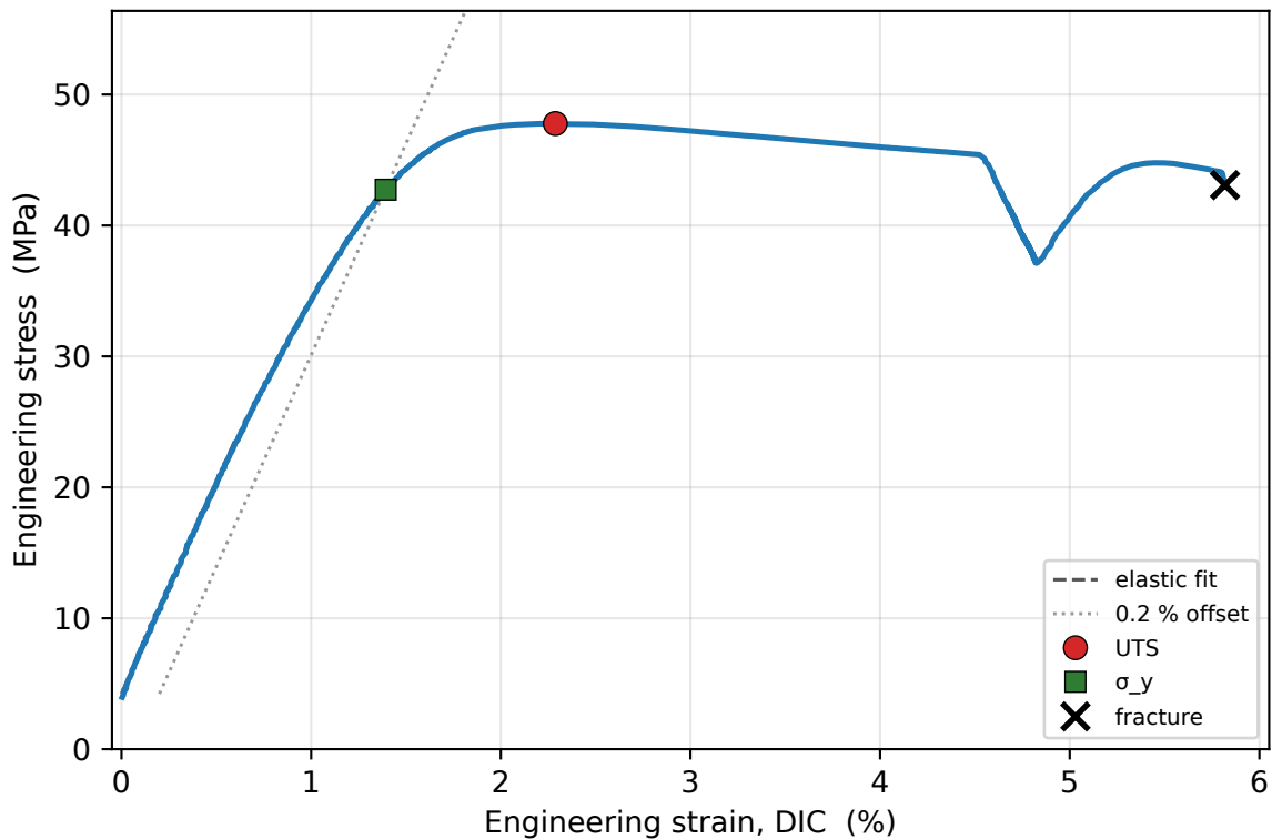
Stress-strain
